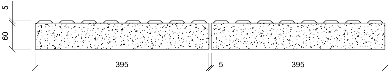
TACTILE WARNING BLOCK 400 x 400 x 65mm THICK
