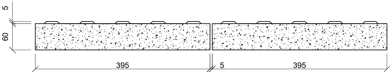
TACTILE DIRECTIONAL BLOCK 400 x 400 x 65mm THICK
