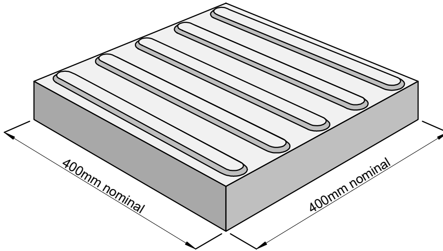
TACTILE WARNING BLOCK 400 x 400 x 65mm THICK
