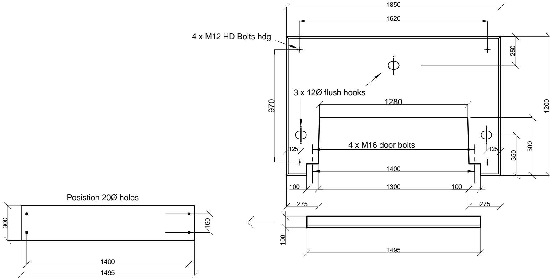
REMOVABLE DOOR
