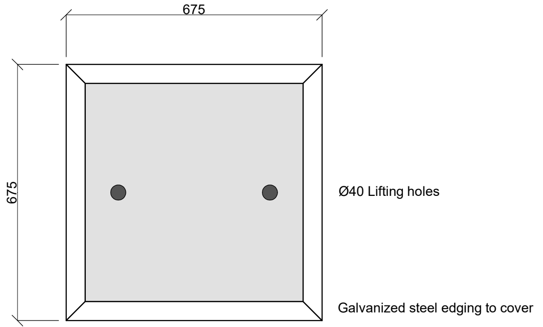
PLAN VIEW
