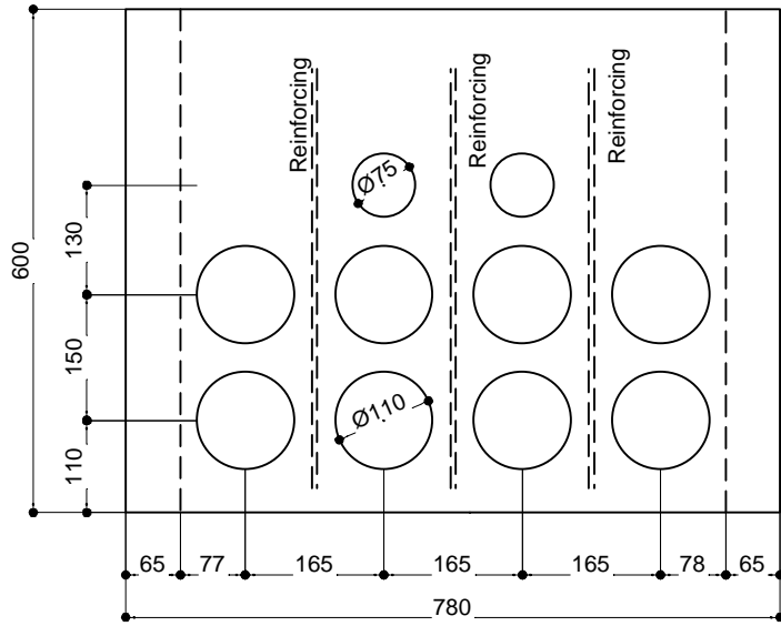
NORTH-SOUTH WALLS
