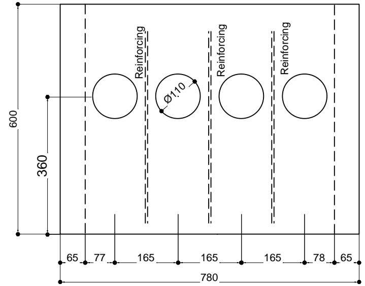
EAST-WEST WALLS
